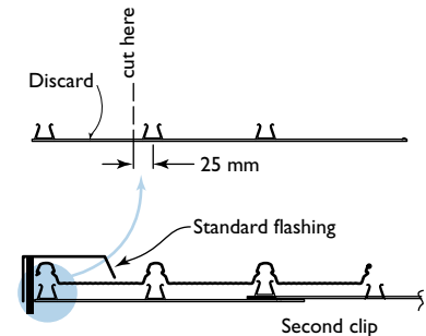
KLIP-LOK 700HS: Starting method 1
